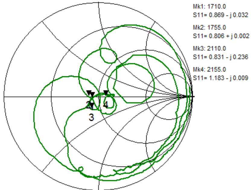
Figure 3-5. Electrical Characteristics
