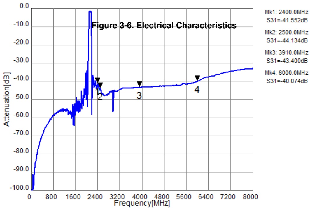
Figure 3-6. Electrical Characteristics
