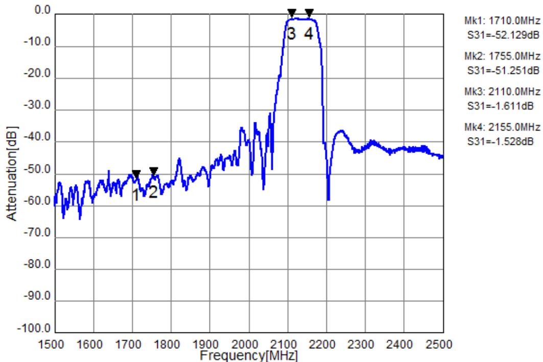
Figure 3-1. Electrical Characteristics
